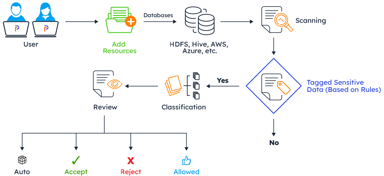
Figure 4: Privacera Data Discovery workflow
